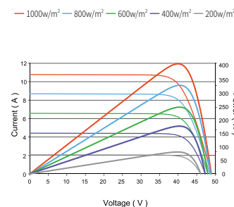
Current-Voltage & Power-Voltage Curves (410W)
