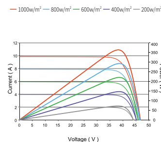
Current-Voltage & Power-Voltage Curves (360W)
